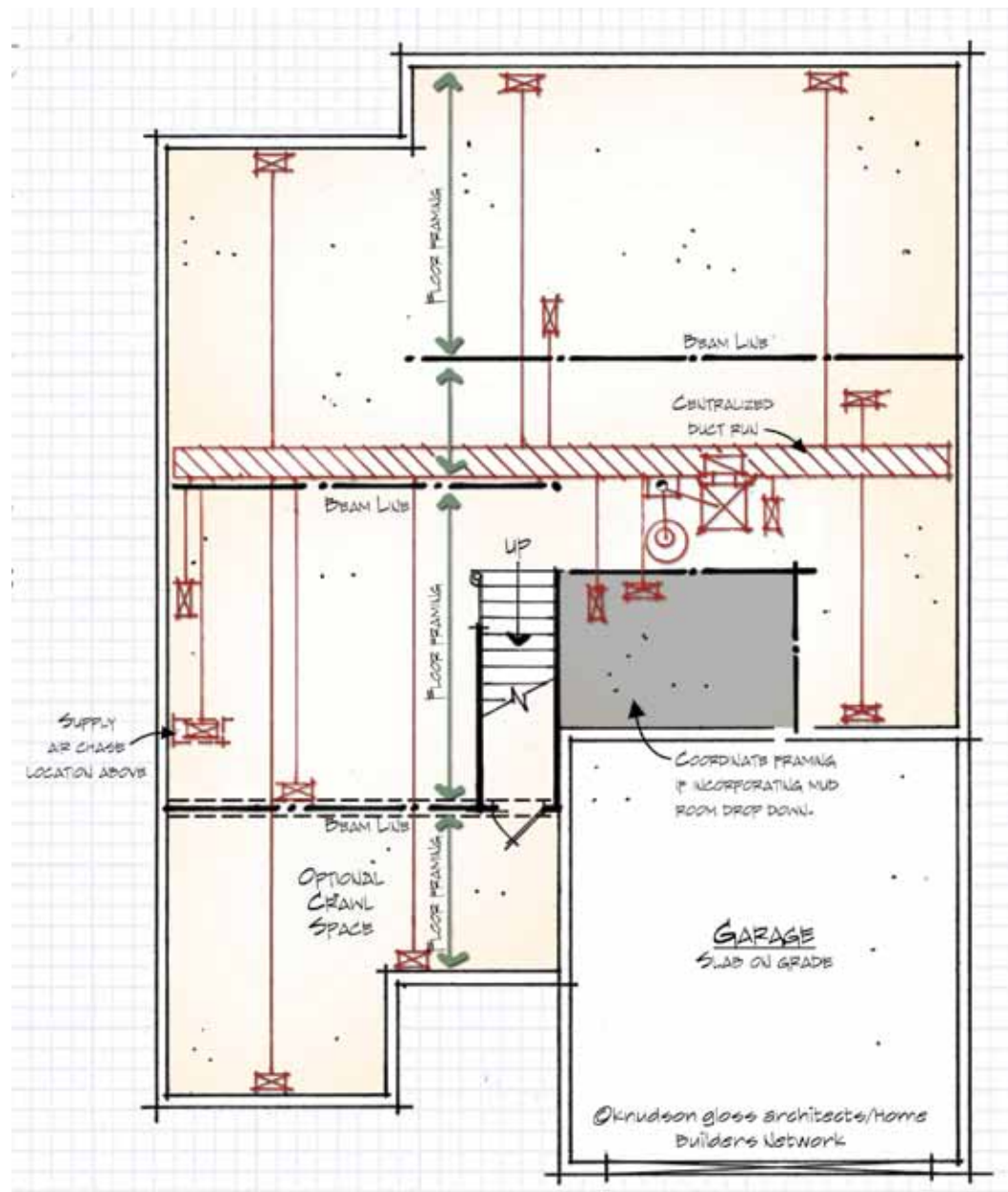
BASEMENT PLAN
