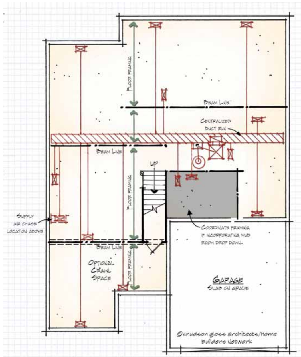
BASEMENT PLAN
