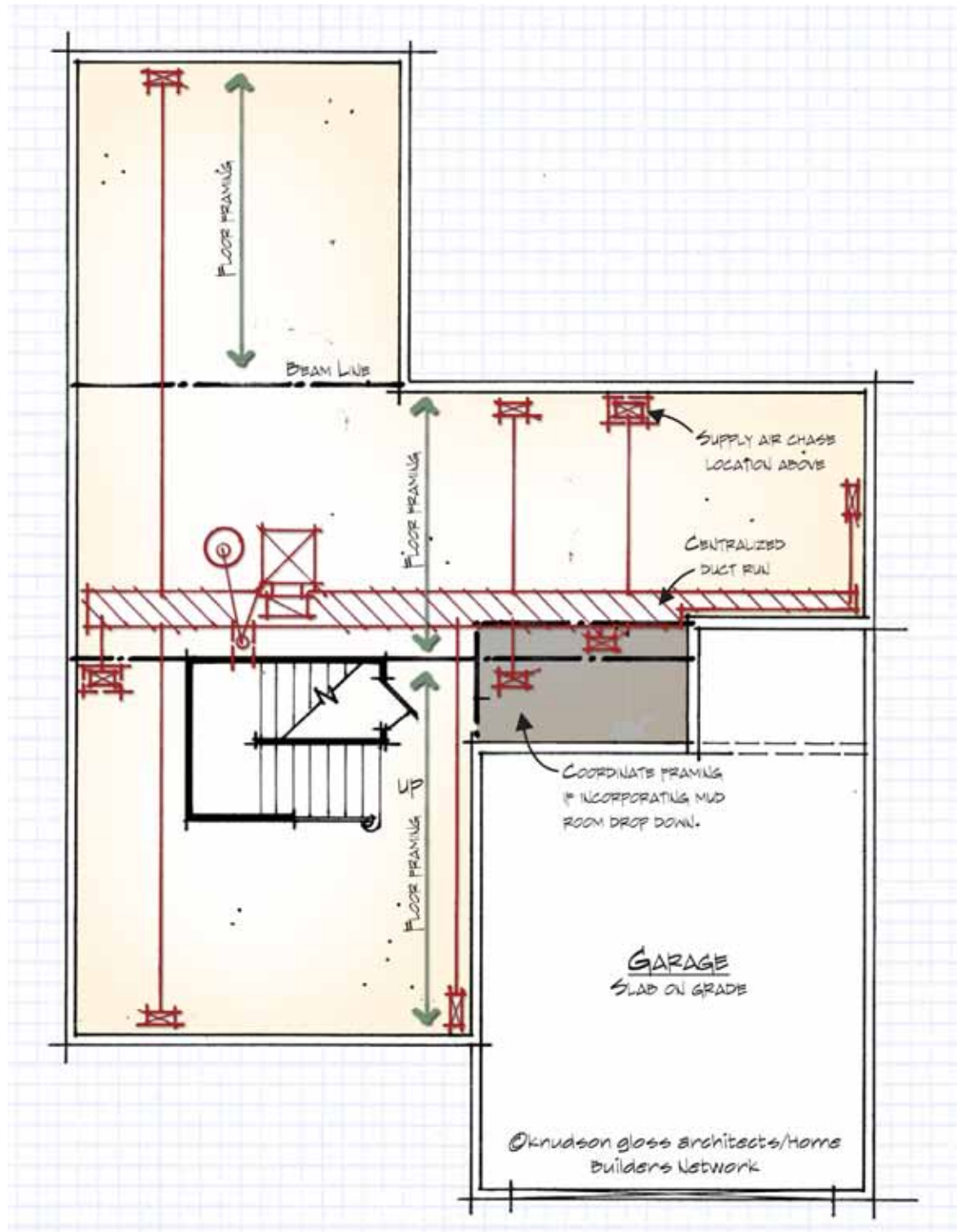
BASEMENT PLAN
