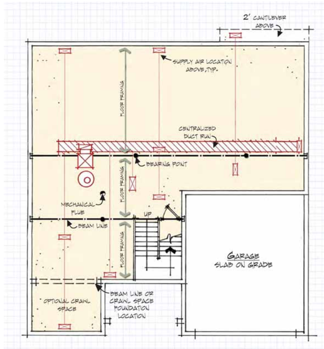
BASEMENT PLAN
