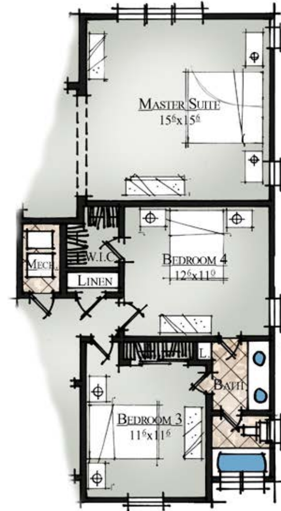
OPTIONAL MASTER SUITE AND BEDROOM 4
